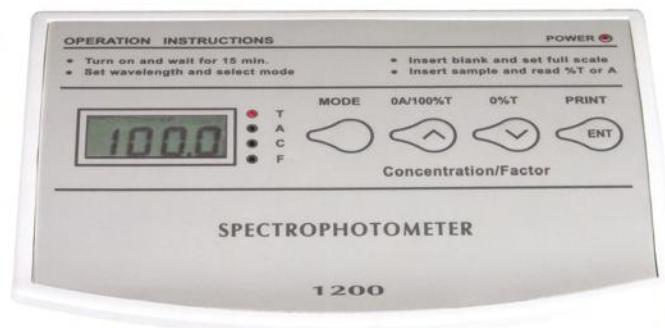
Close-up view of S1200 instrument panel
